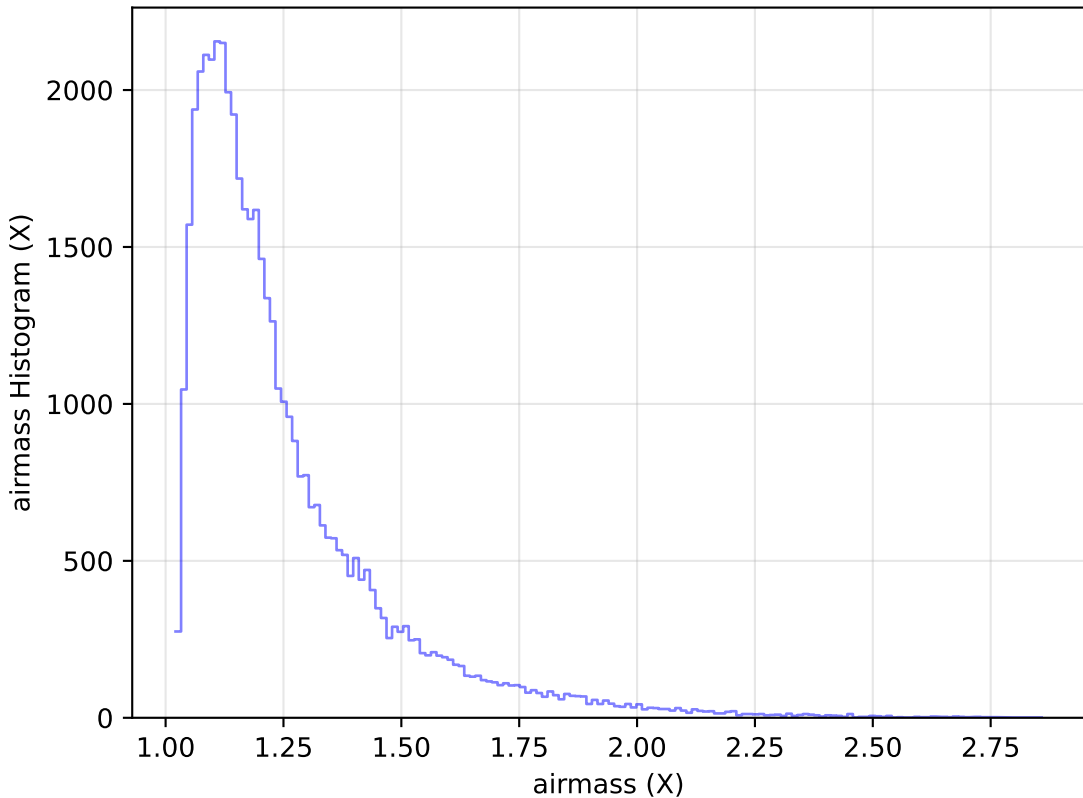
too_elab_r64_d2_giz_v3.4_10yrs Yr 1 y band: airmass Histogram
