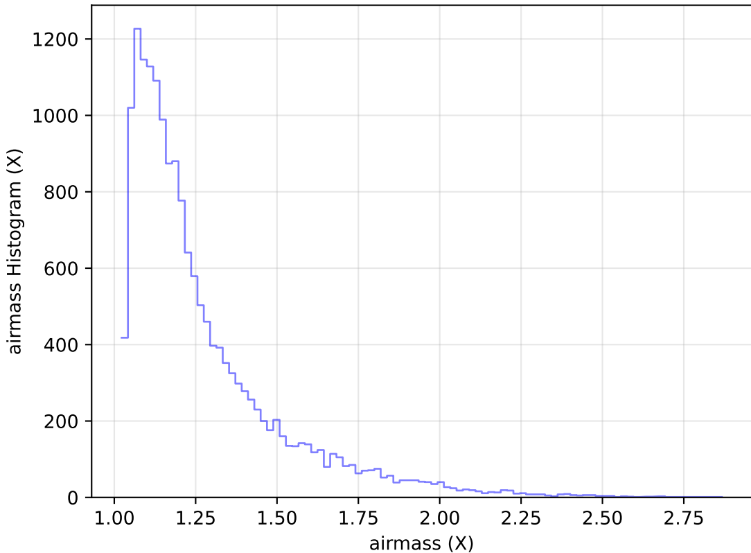
too_elab_r64_d2_giz_v3.4_10yrs Yr 1 u band: airmass Histogram
