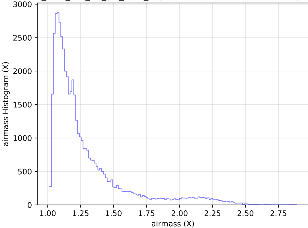
too_elab_r64_d2_giz_v3.4_10yrs Yr 1 r band: airmass Histogram
