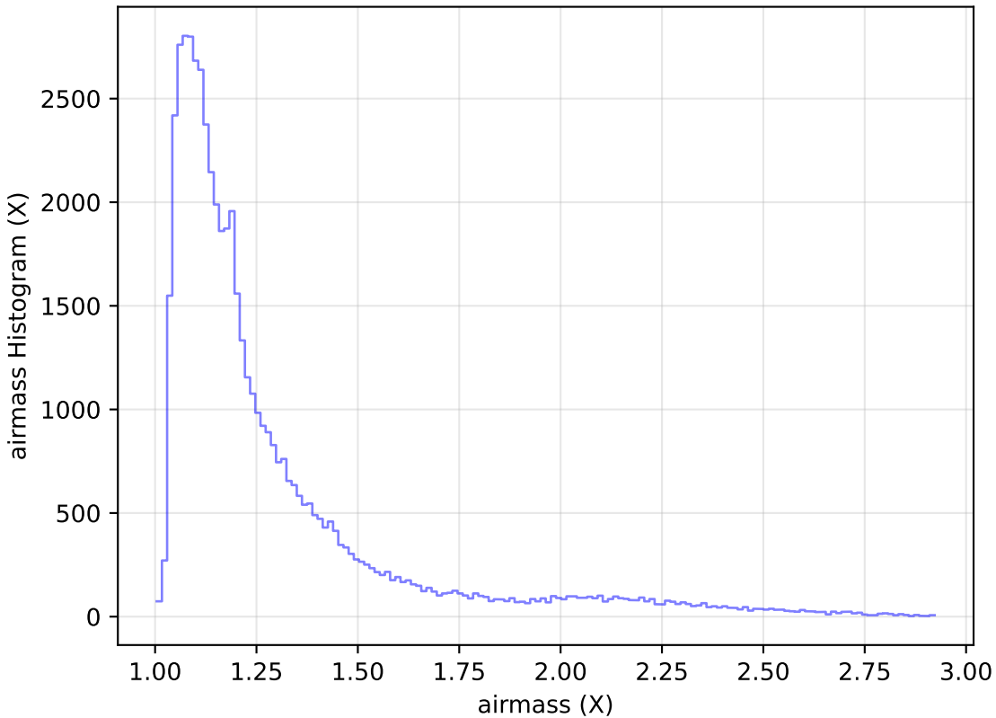
too_elab_r64_d2_giz_v3.4_10yrs Yr 1 i band: airmass Histogram
