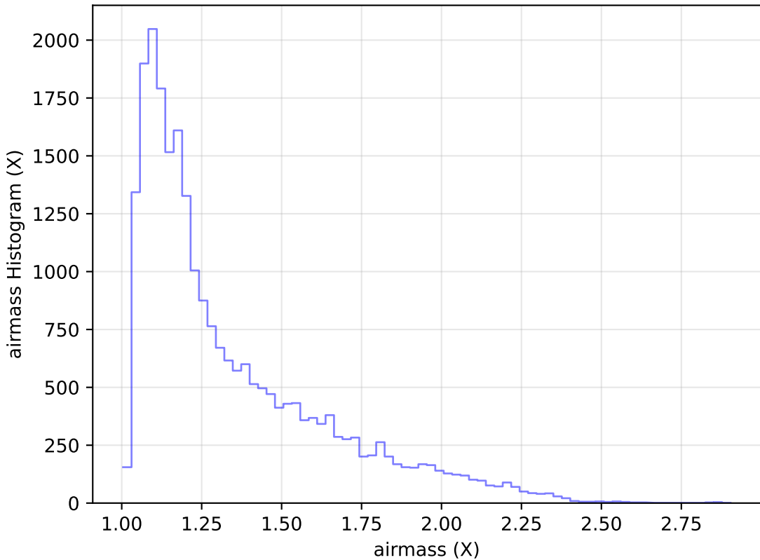
too_elab_r64_d2_giz_v3.4_10yrs Yr 1 g band: airmass Histogram
