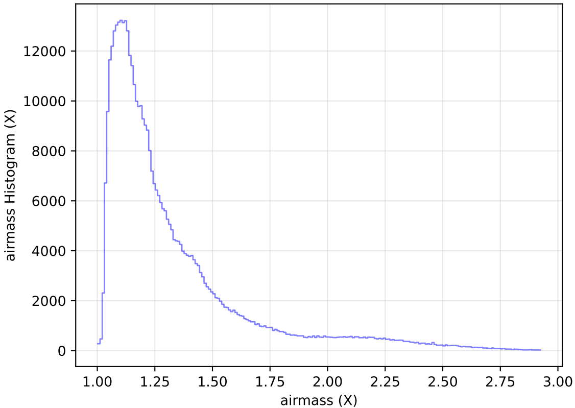
too_elab_r64_d2_giz_v3.4_10yrs WFD z band: airmass Histogram
