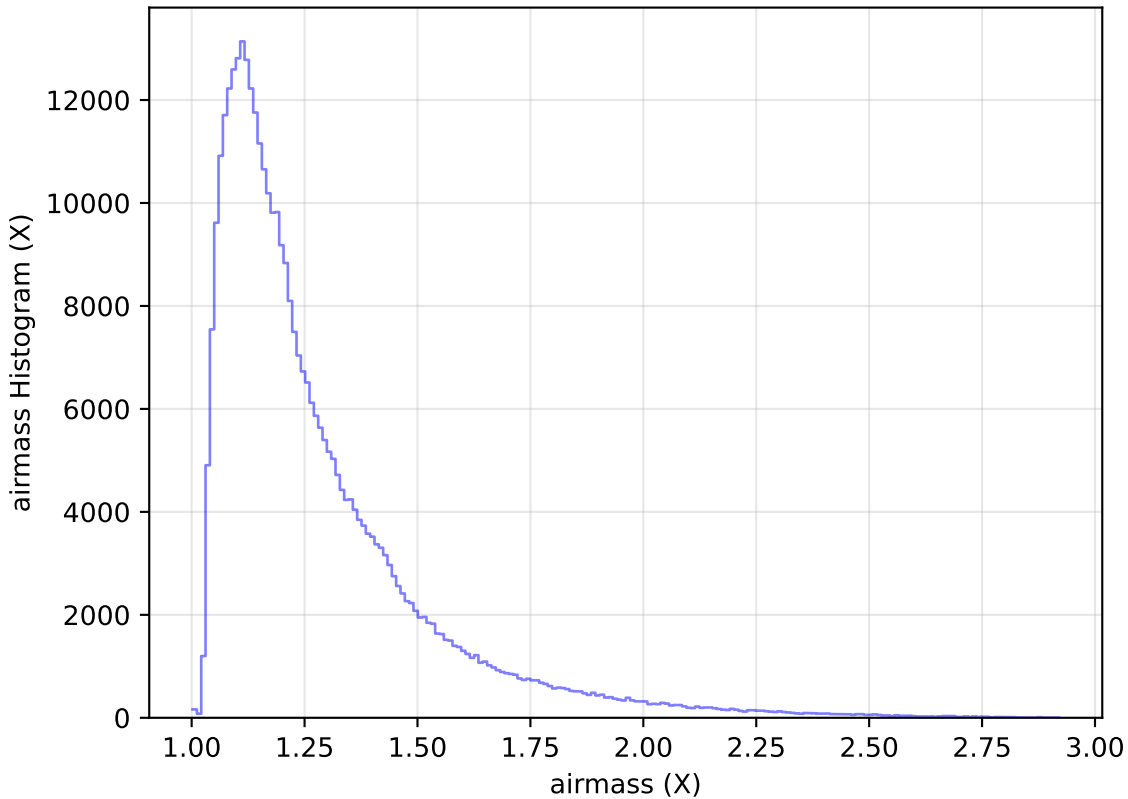
too_elab_r64_d2_giz_v3.4_10yrs WFD y band: airmass Histogram
