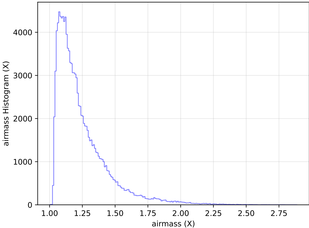
too_elab_r64_d2_giz_v3.4_10yrs WFD u band: airmass Histogram
