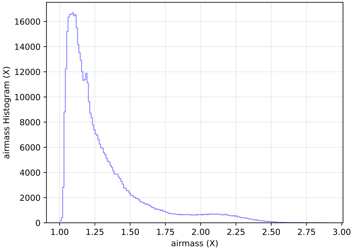
too_elab_r64_d2_giz_v3.4_10yrs WFD r band: airmass Histogram
