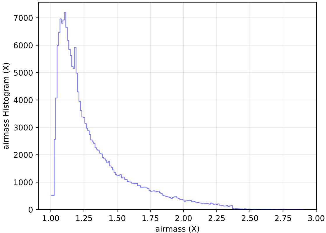
too_elab_r64_d2_giz_v3.4_10yrs WFD g band: airmass Histogram
