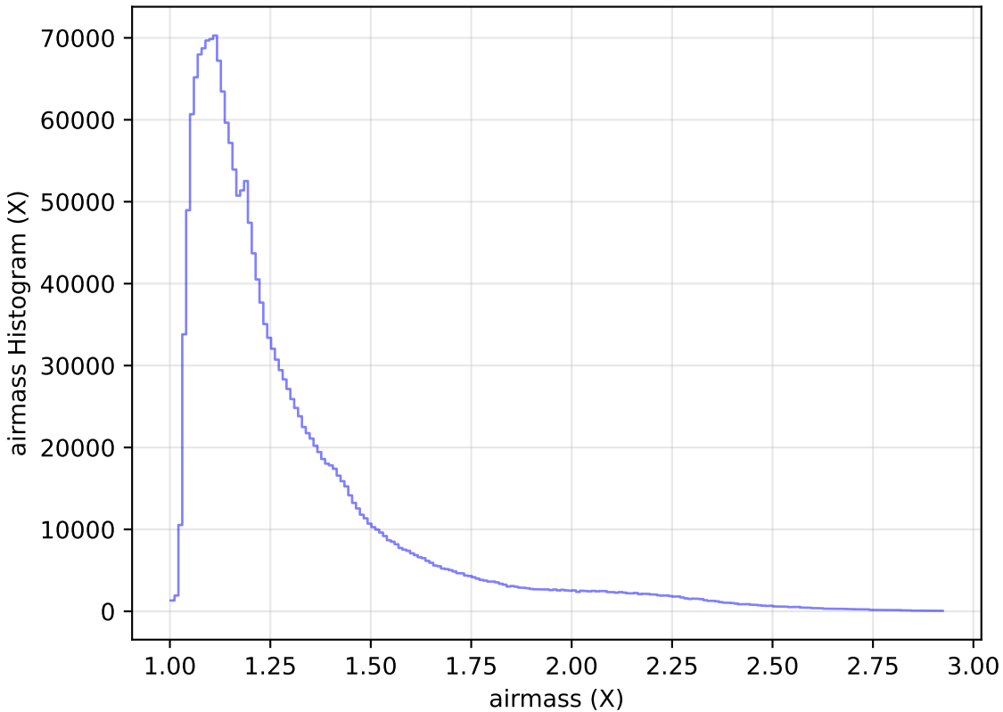
too_elab_r64_d2_giz_v3.4_10yrs WFD all bands: airmass Histogram
