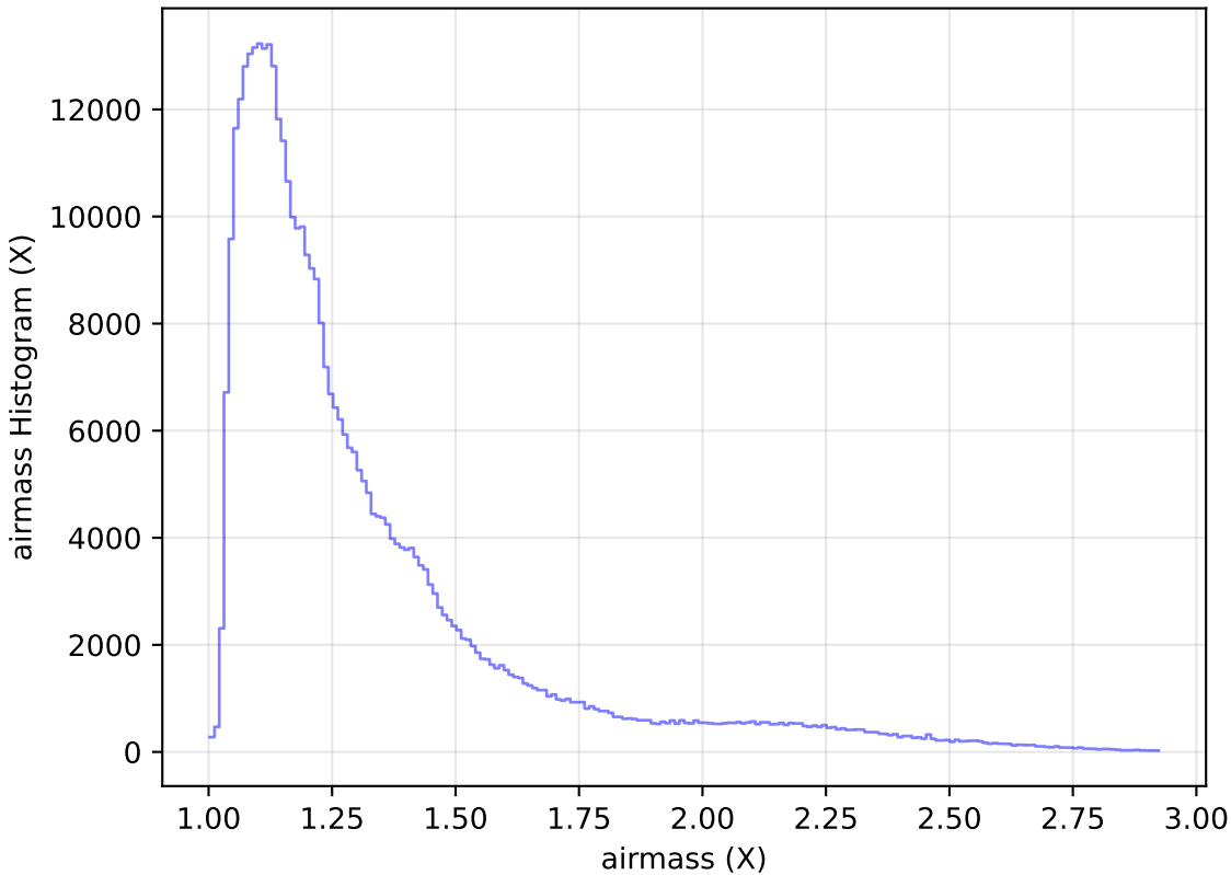
too_elab_r64_d2_giz_v3.4_10yrs All sky z band: airmass Histogram
