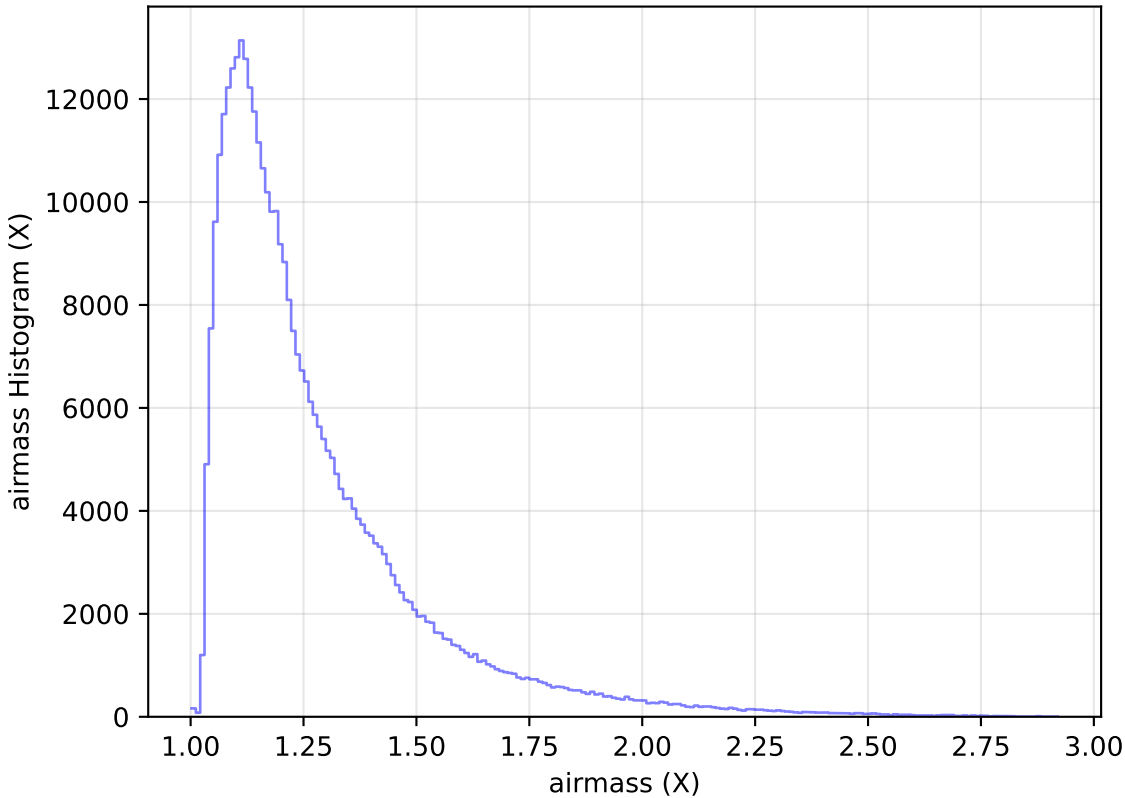
too_elab_r64_d2_giz_v3.4_10yrs All sky y band: airmass Histogram
