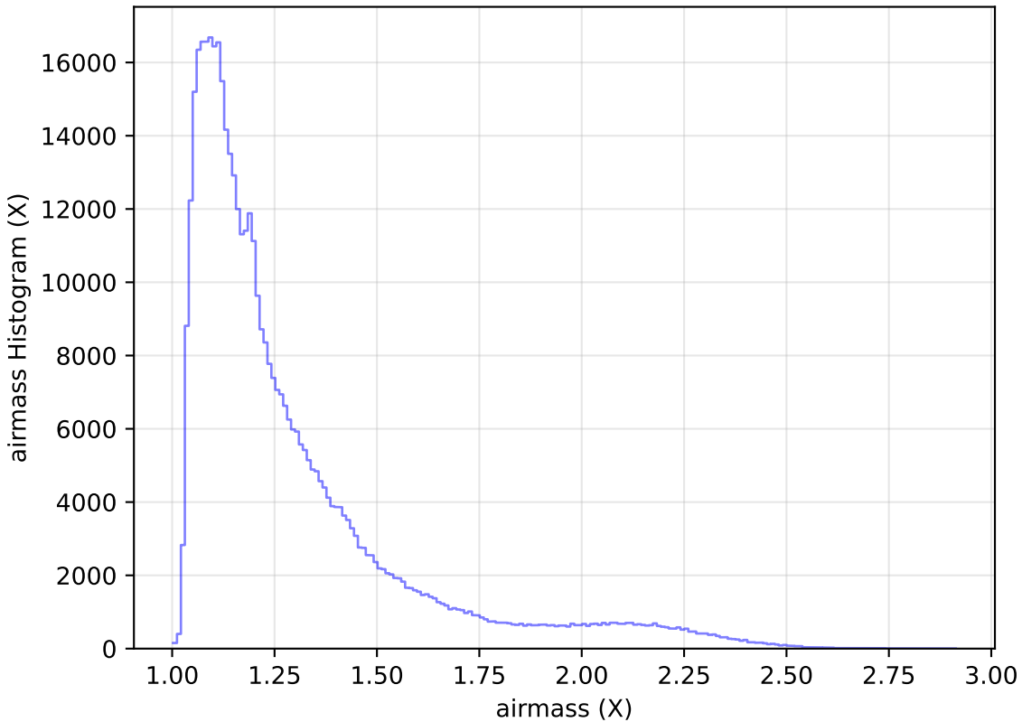
too_elab_r64_d2_giz_v3.4_10yrs All sky r band: airmass Histogram
