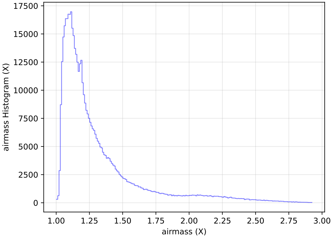
too_elab_r64_d2_giz_v3.4_10yrs All sky i band: airmass Histogram
