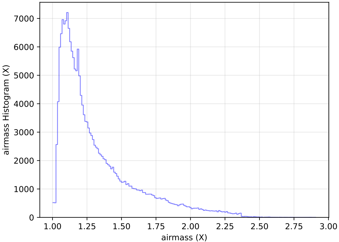
too_elab_r64_d2_giz_v3.4_10yrs All sky g band: airmass Histogram
