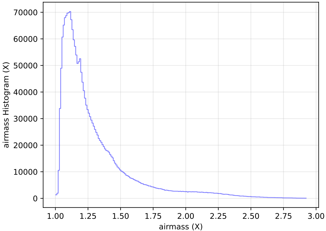
too_elab_r64_d2_giz_v3.4_10yrs All sky all bands: airmass Histogram
