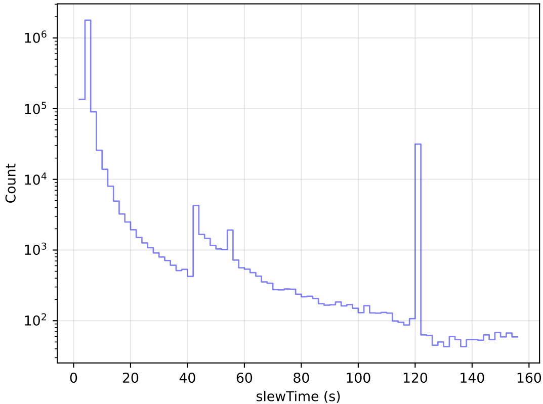
too_elab_r64_d2_giz_v3.4_10yrs All visits: Slew Time Histogram
