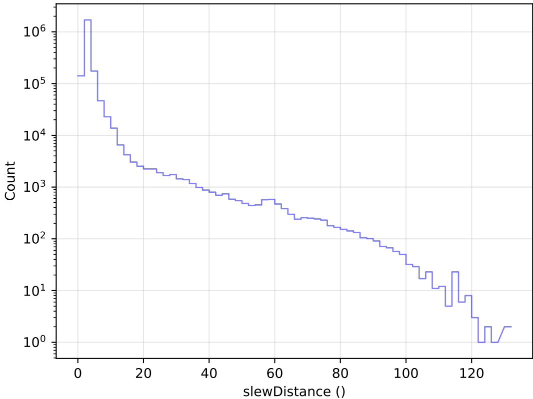
too_elab_r64_d2_giz_v3.4_10yrs All visits: Slew Distance Histogram
