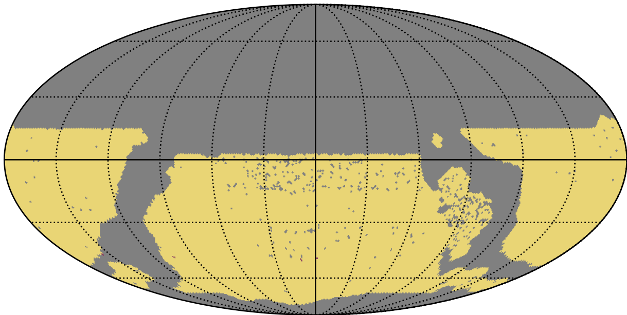
too_elab_r64_d2_giz_v3.4_10yrs WFD: RapidRevisits
