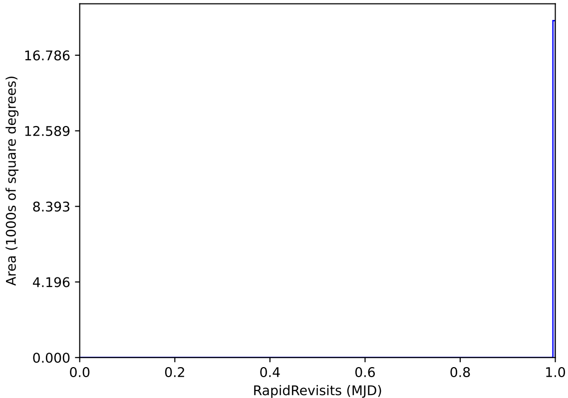
too_elab_r64_d2_giz_v3.4_10yrs WFD: RapidRevisits
