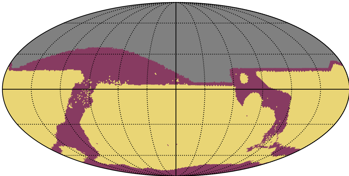
too_elab_r64_d2_giz_v3.4_10yrs All sky: RapidRevisits
