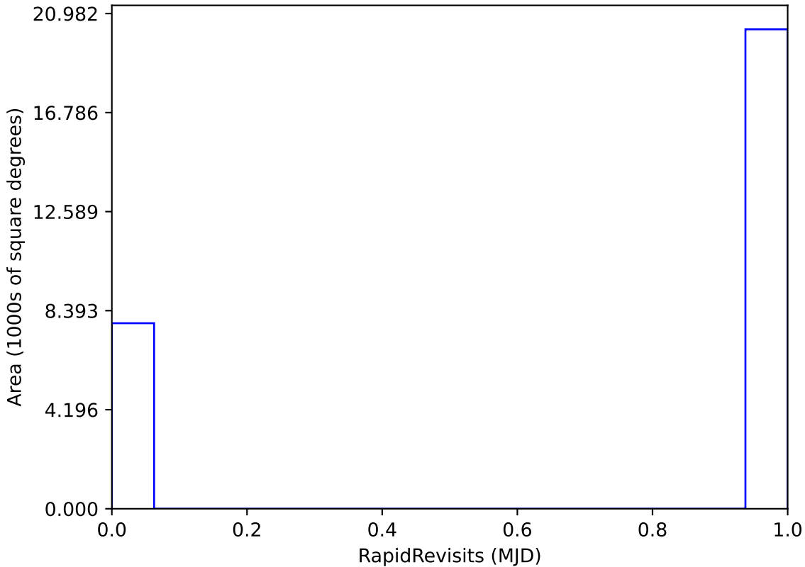
too_elab_r64_d2_giz_v3.4_10yrs All sky: RapidRevisits
