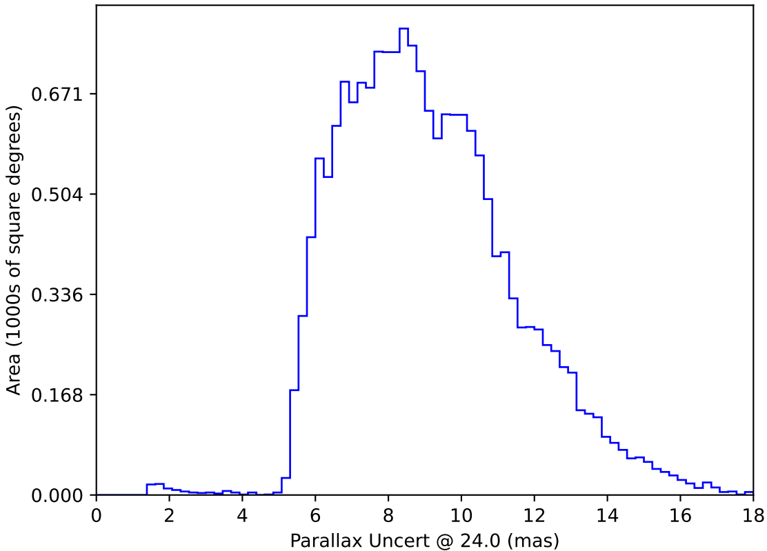
too_elab_r64_d2_giz_v3.4_10yrs WFD: Parallax Uncert @ 24.0
