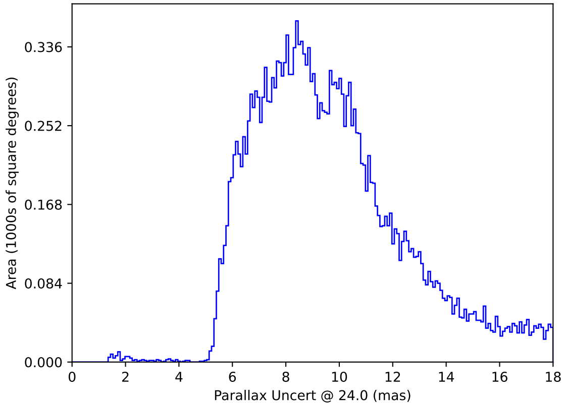
too_elab_r64_d2_giz_v3.4_10yrs All sky: Parallax Uncert @ 24.0
