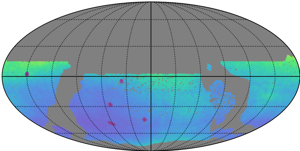
too_elab_r64_d2_giz_v3.4_10yrs WFD: Parallax Uncert @ 22.4
