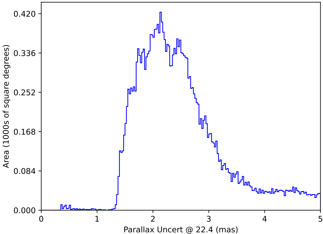
too_elab_r64_d2_giz_v3.4_10yrs All sky: Parallax Uncert @ 22.4
