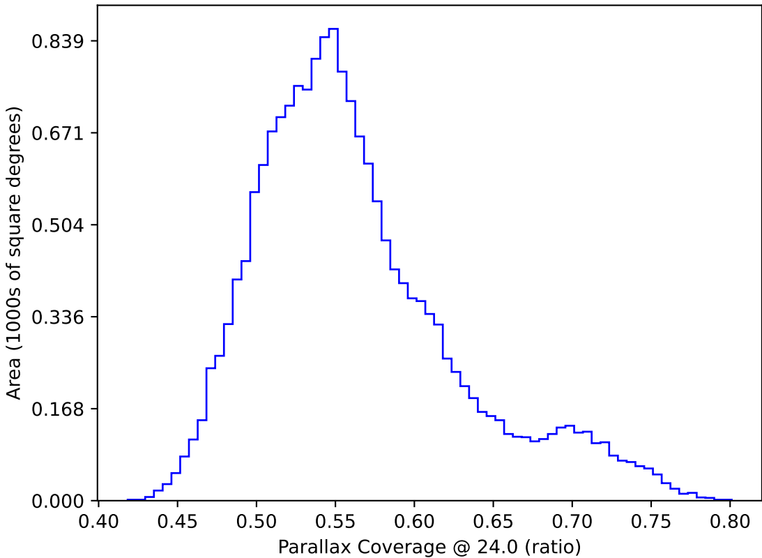
too_elab_r64_d2_giz_v3.4_10yrs WFD: Parallax Coverage @ 24.0
