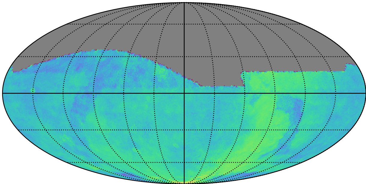
too_elab_r64_d2_giz_v3.4_10yrs All sky: Parallax Coverage @ 24.0
