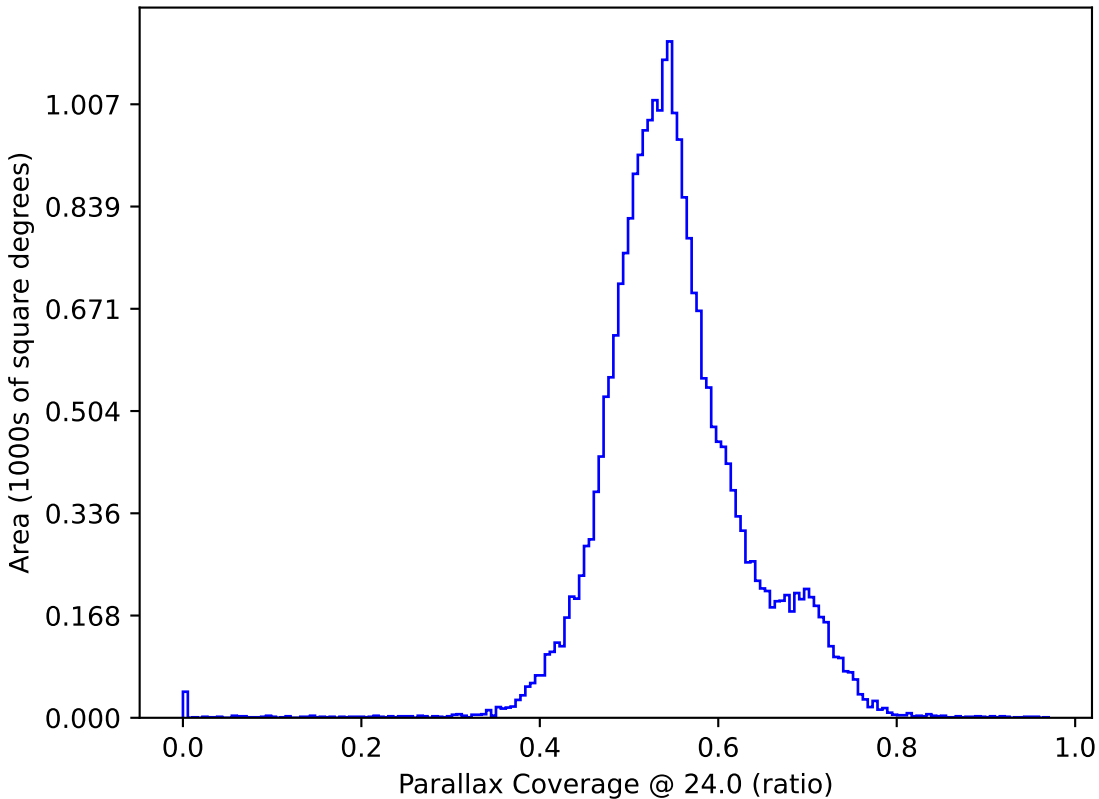
too_elab_r64_d2_giz_v3.4_10yrs All sky: Parallax Coverage @ 24.0
