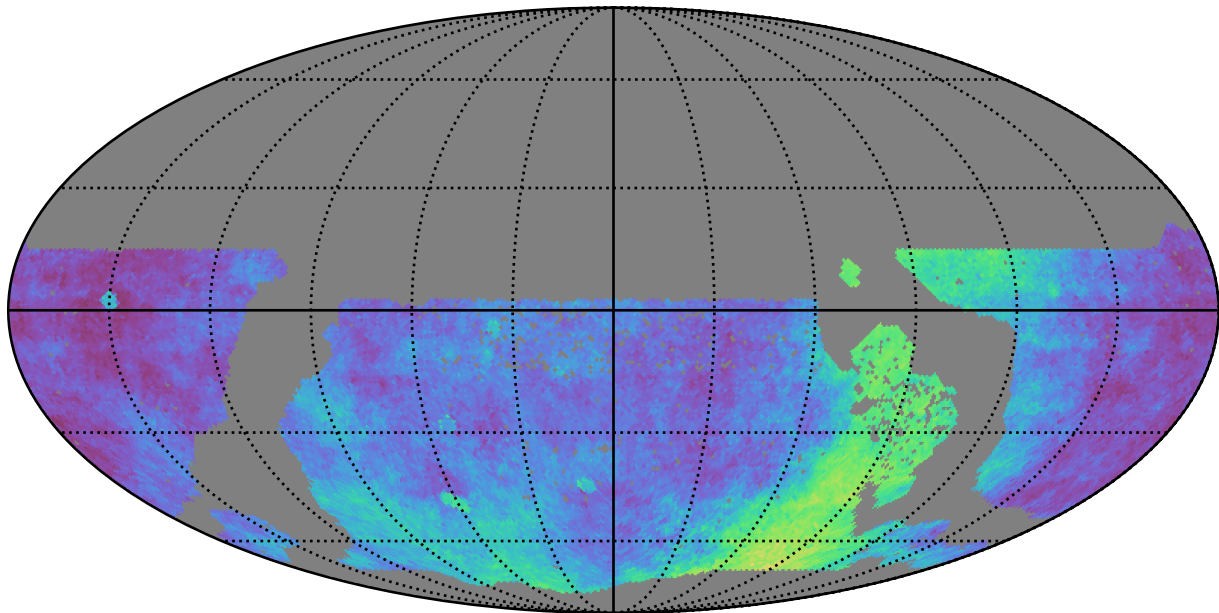
too_elab_r64_d2_giz_v3.4_10yrs WFD: Parallax Coverage @ 22.4
