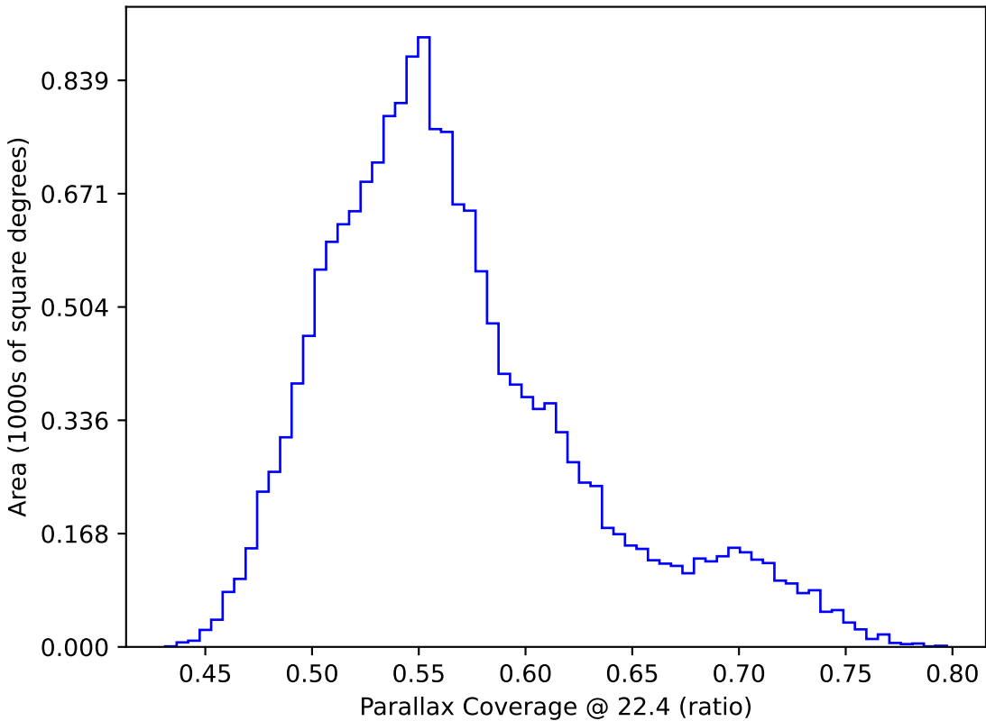
too_elab_r64_d2_giz_v3.4_10yrs WFD: Parallax Coverage @ 22.4
