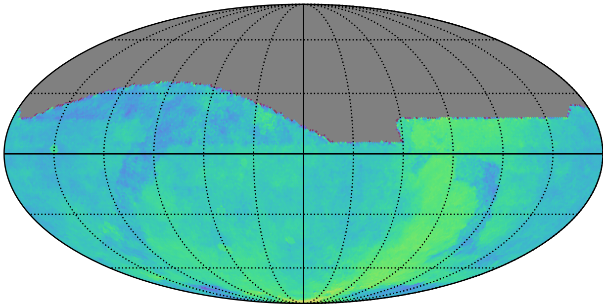
too_elab_r64_d2_giz_v3.4_10yrs All sky: Parallax Coverage @ 22.4
