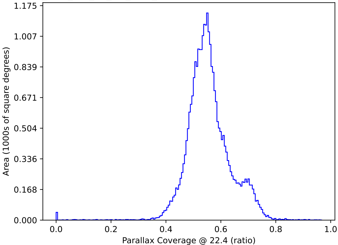
too_elab_r64_d2_giz_v3.4_10yrs All sky: Parallax Coverage @ 22.4
