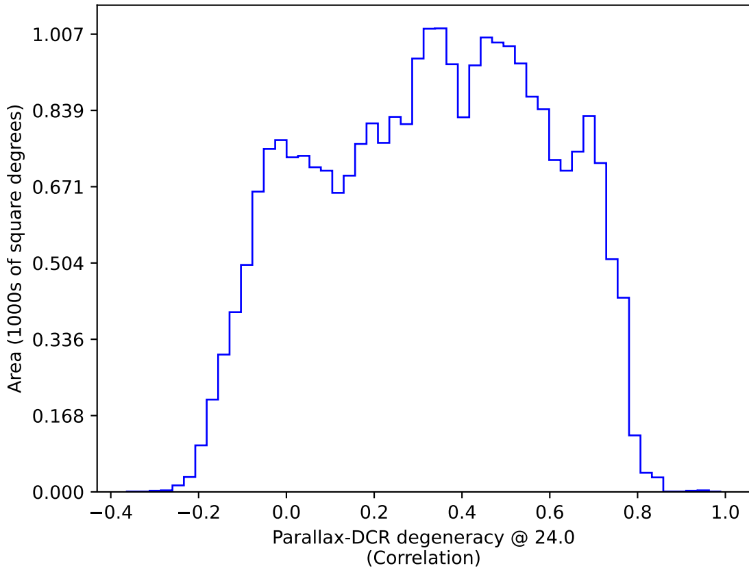
too_elab_r64_d2_giz_v3.4_10yrs All sky: Parallax-DCR degeneracy @ 24.0
