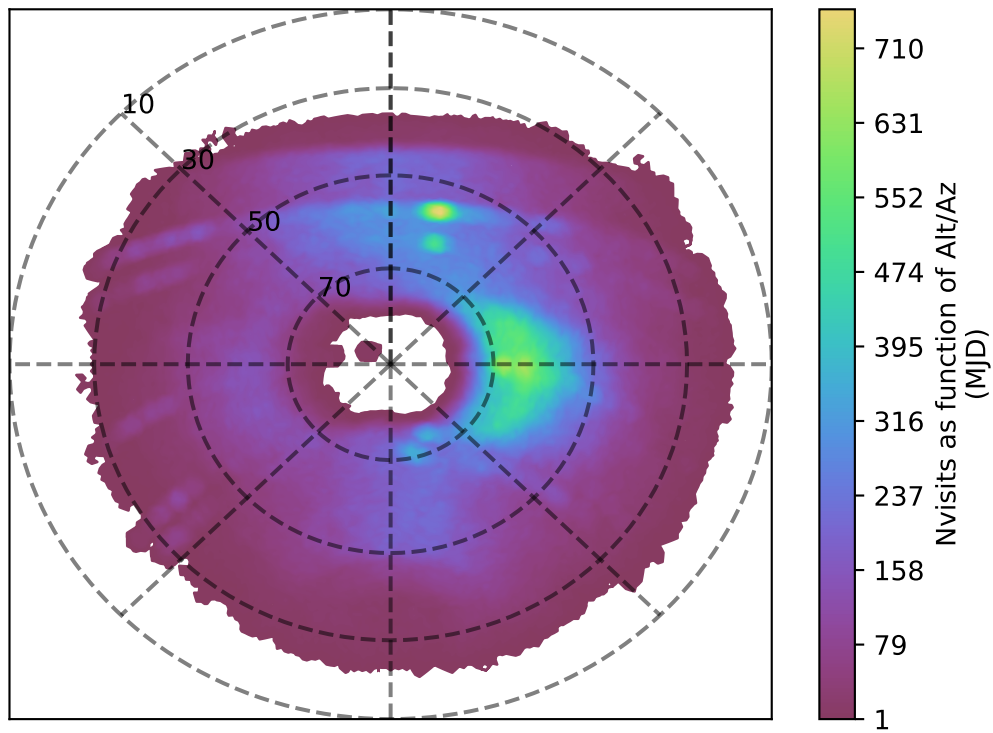
too_elab_r64_d2_giz_v3.4_10yrs u band: Nvisits as function of Alt/Az
