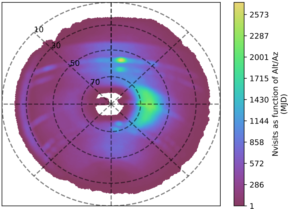
too_elab_r64_d2_giz_v3.4_10yrs r band: Nvisits as function of Alt/Az
