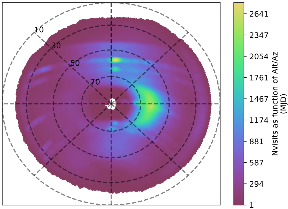
too_elab_r64_d2_giz_v3.4_10yrs i band: Nvisits as function of Alt/Az
