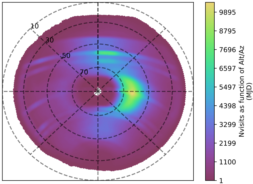
too_elab_r64_d2_giz_v3.4_10yrs all bands: Nvisits as function of Alt/Az
