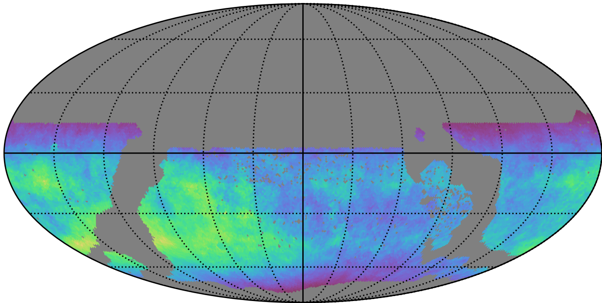
too_elab_r64_d2_giz_v3.4_10yrs WFD z band: Normalized Teff
