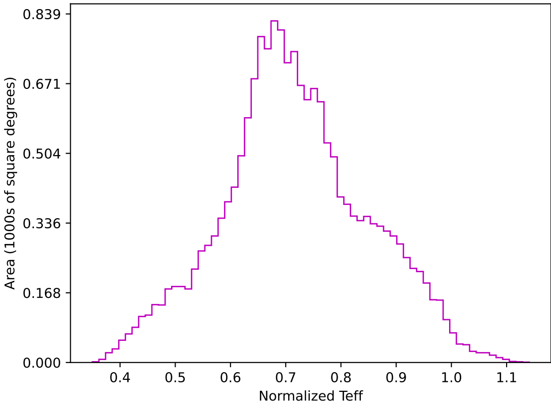
too_elab_r64_d2_giz_v3.4_10yrs WFD z band: Normalized Teff
