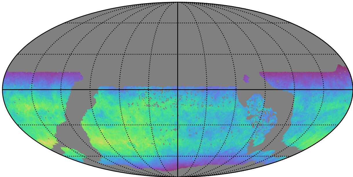
too_elab_r64_d2_giz_v3.4_10yrs WFD y band: Normalized Teff
