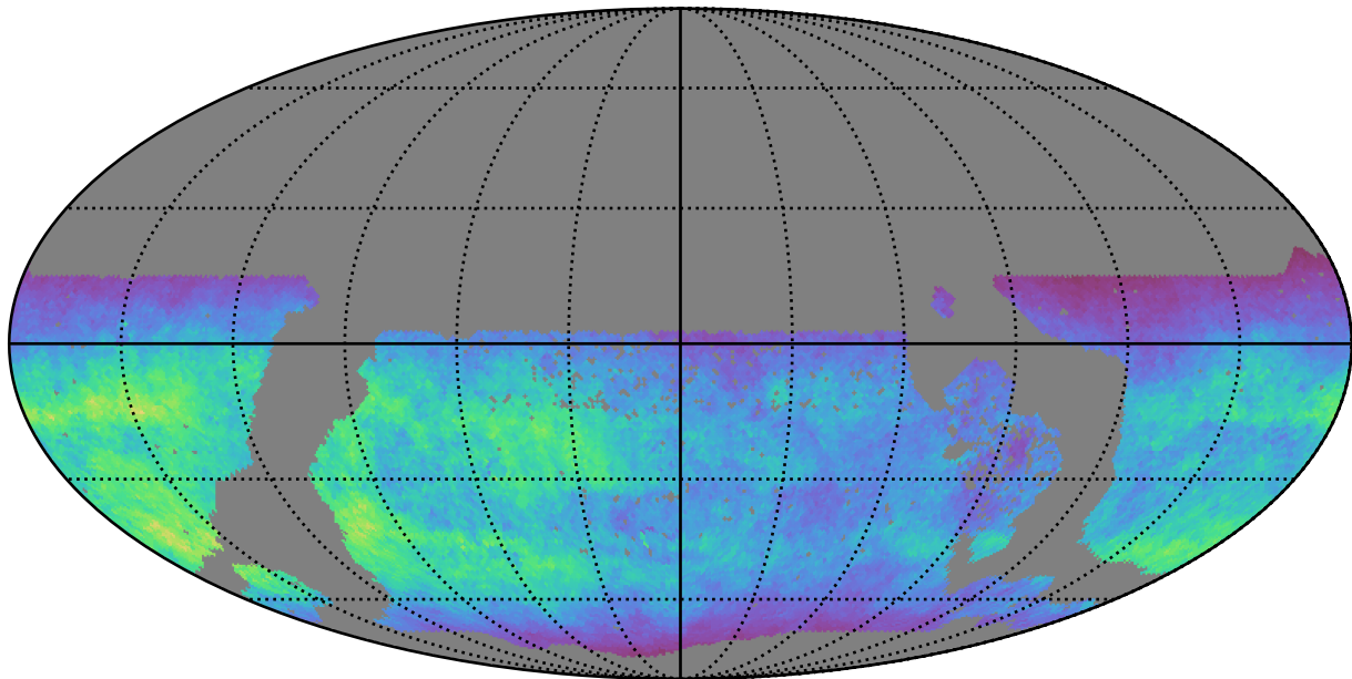
too_elab_r64_d2_giz_v3.4_10yrs WFD u band: Normalized Teff
