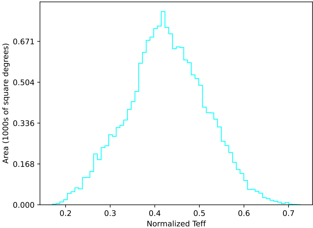
too_elab_r64_d2_giz_v3.4_10yrs WFD u band: Normalized Teff
