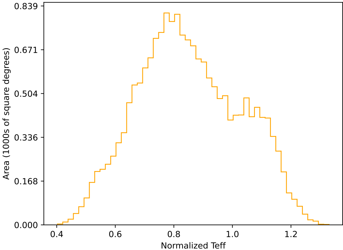
too_elab_r64_d2_giz_v3.4_10yrs WFD r band: Normalized Teff
