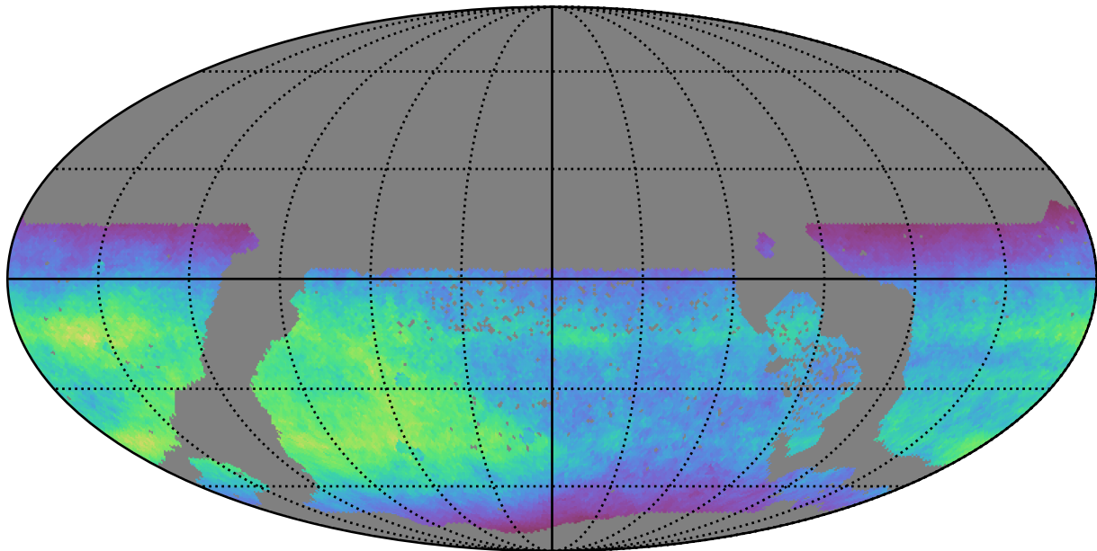
too_elab_r64_d2_giz_v3.4_10yrs WFD i band: Normalized Teff
