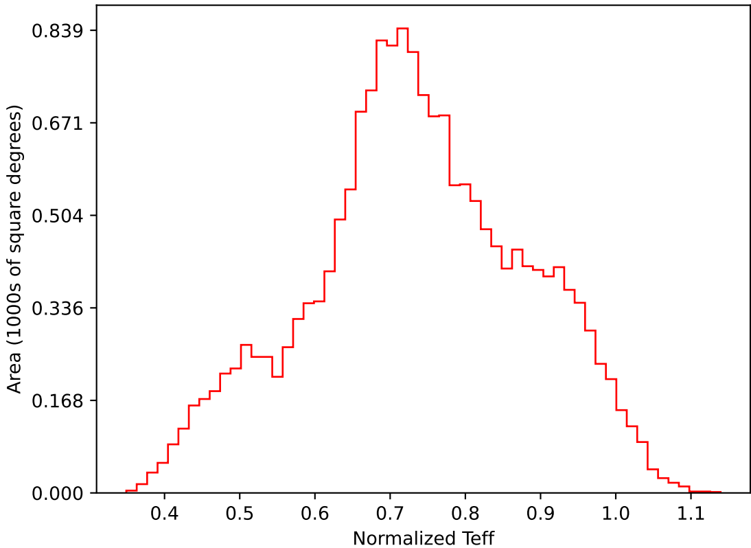
too_elab_r64_d2_giz_v3.4_10yrs WFD i band: Normalized Teff
