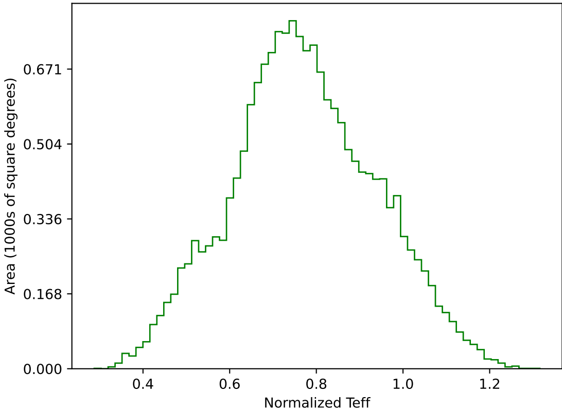
too_elab_r64_d2_giz_v3.4_10yrs WFD g band: Normalized Teff
