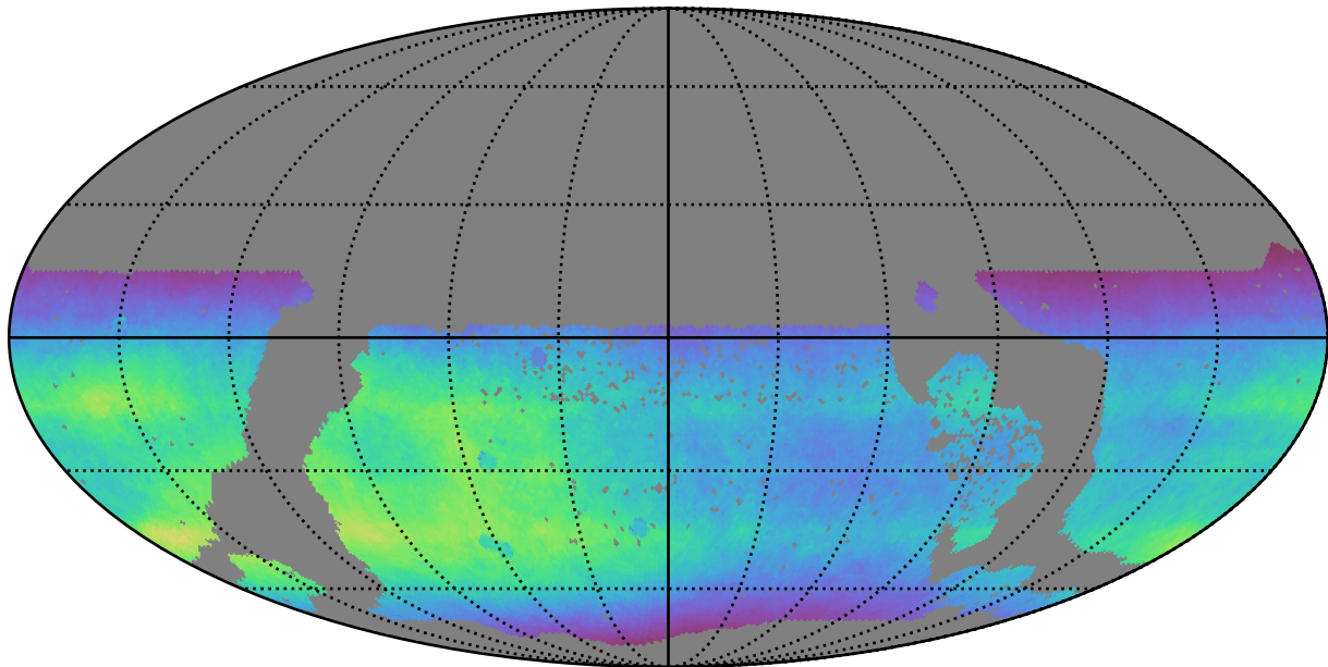
too_elab_r64_d2_giz_v3.4_10yrs WFD all bands: Normalized Teff
