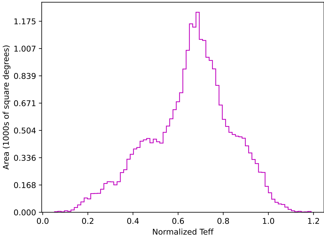
too_elab_r64_d2_giz_v3.4_10yrs All sky z band: Normalized Teff
